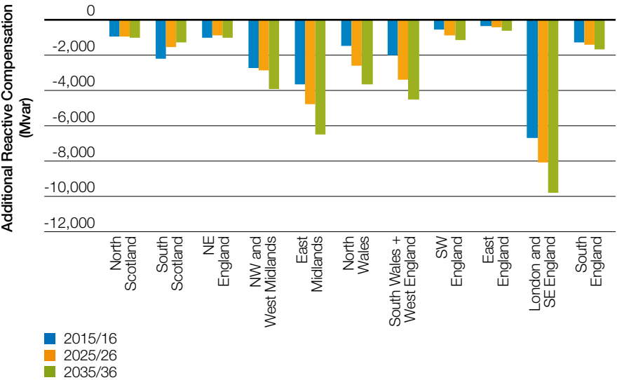
Figure 51 Regional Breakdown of Additional Requirements for Reactive Compensation
