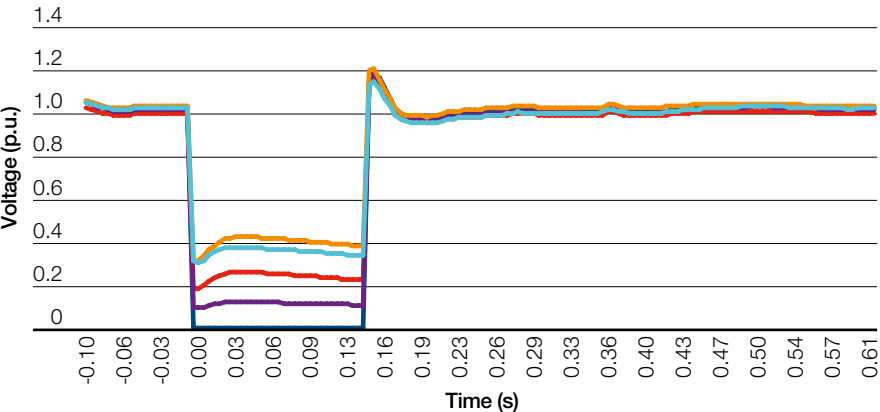
Figure 34 2025 Gone Green 3-phase Earth Fault at Walpole 400kV Transient Voltage Dip Event
