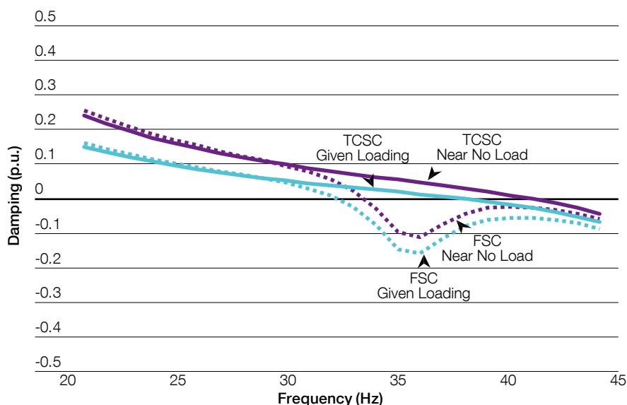
Figure 82 Electrical Damping Versus Torsional Frequencies for Different Loadings (FSC without SSR filter, TCSC and SSR control)
