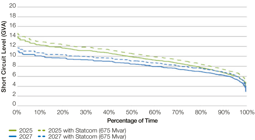
Figure 57 Load Duration Assessment of Sellindge 400kV System Strength against SCL and Effective SCL with STATCOM (2015 Assessment)
