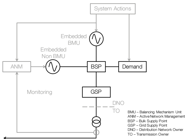
Figure 75 Type-D ANM Architecture
