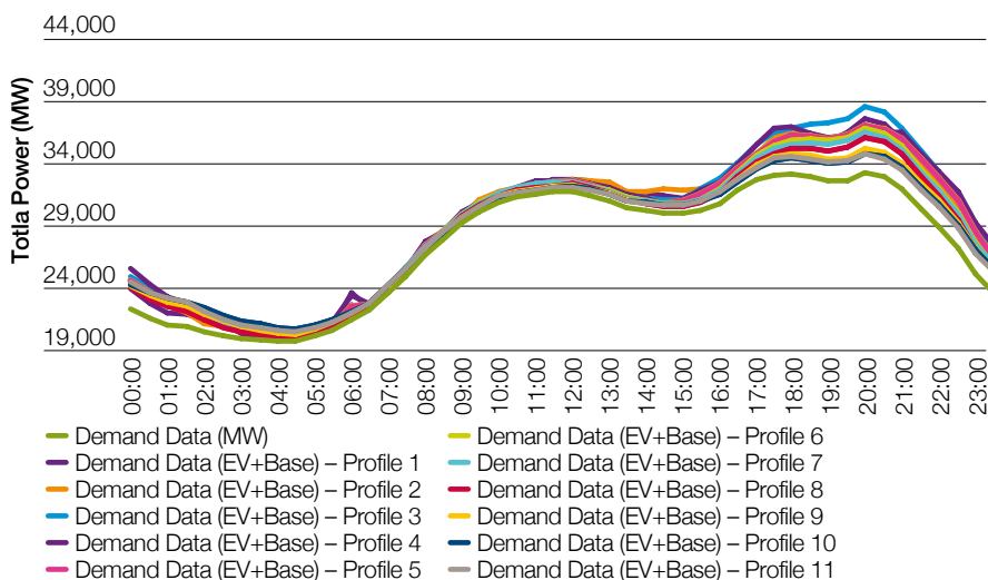
Figure 87 Impact of Electric Vehicles on Daily Load Profile
