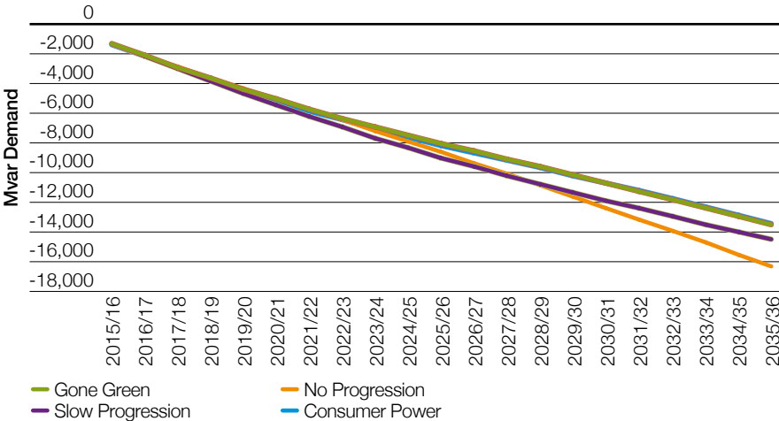
Figure 47 Projected GSP Reactive Power Exchange
