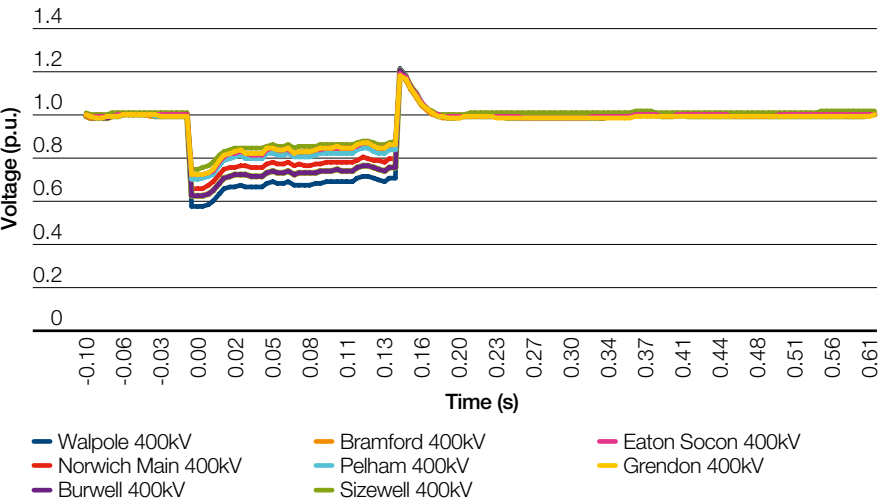
Figure 36 2025 Gone Green Single-phase to Earth Fault at Walpole 400kV Transient Voltage Dip Event
