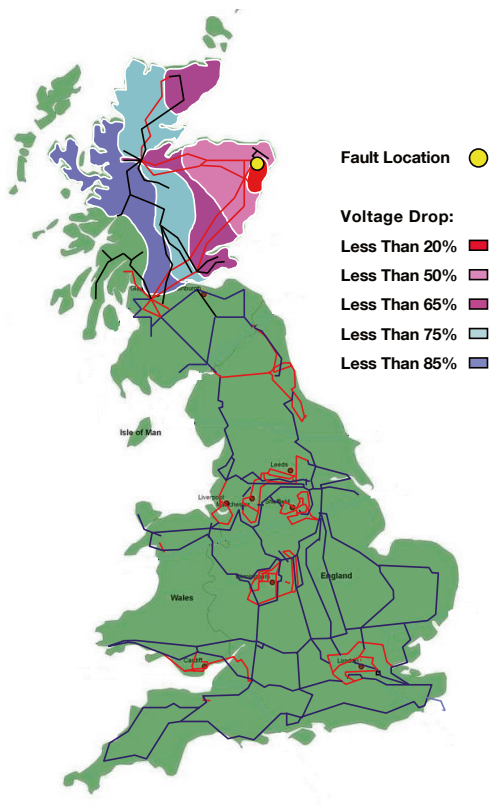
Figure 29 Voltage Dip Spread Example (2014/15 Fault at Peterhead)
