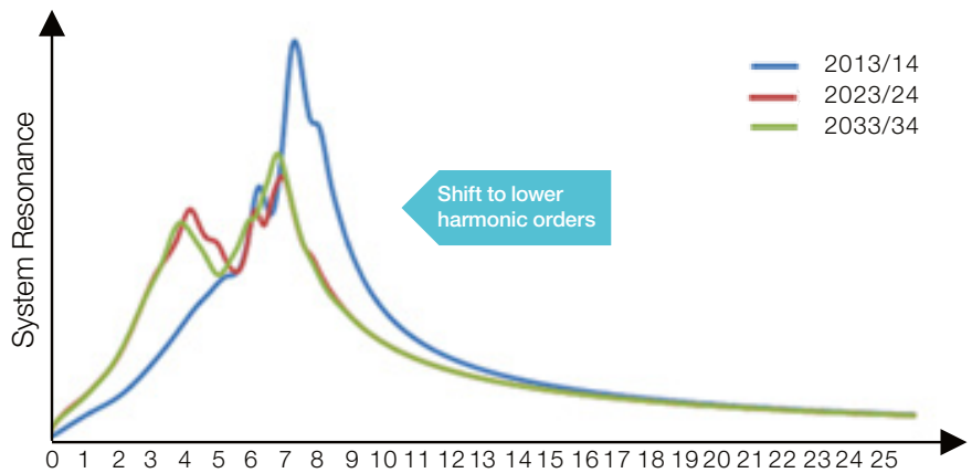
Figure 52 Illustration of Lower Order Harmonic Shift
