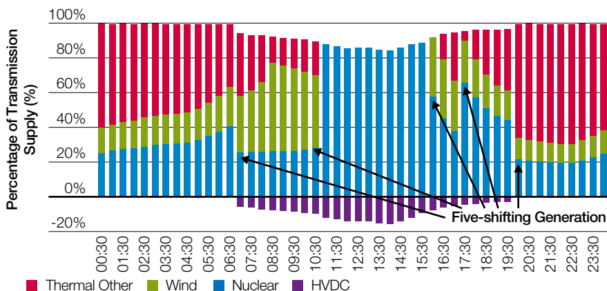
Figure 28C 2035 Thermal Generation Shifting Against FES 2015 Balancing Case Stud
