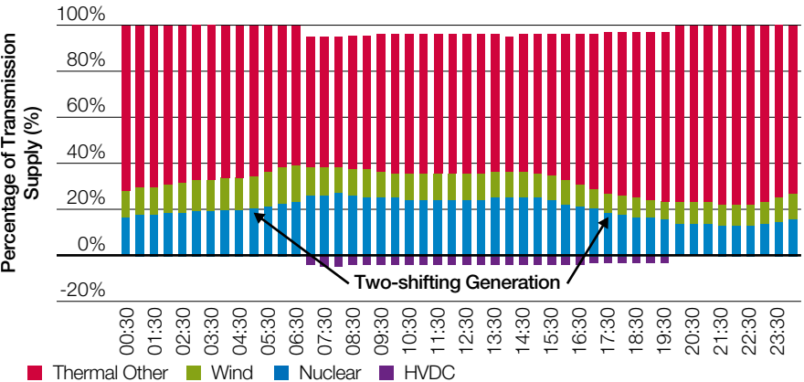
Figure 28A 2020 Thermal Generation Shifting Against FES 2015 Balancing Case Study
