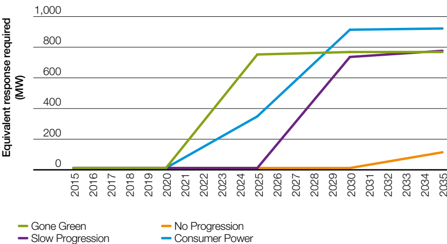
Figure 21 Enhanced Response Requirements After Synchronous Response Has Been Used
