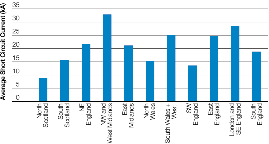
Figure 24 SOF 2015 Regions Short Circuit Level 2015/16
