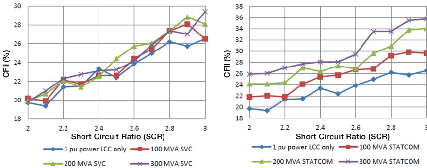
Figure 58 Comparison of CFI with Short Circuit Ratio Noting Influence of Statcom and SVCs
