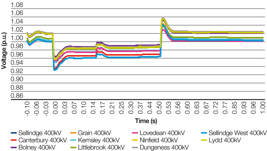
Figure 41 2025 Gone Green Single-phase to Earth Fault at Sellindge 132kV for 500ms
