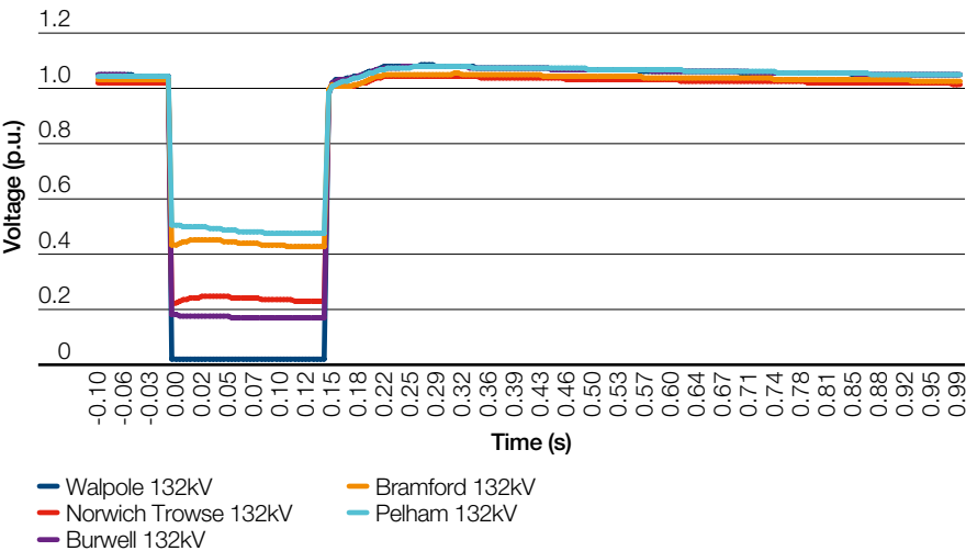
Figure 33 Current Network 3-phase Earth Fault at Walpole 400kV Transient Voltage Dip Event
