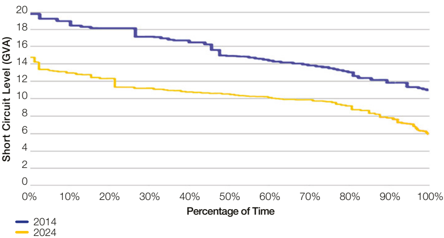
Figure 56 Load Duration Assessment of Sellindge 400kV System Strength Against SCL (2014 Assessment)
