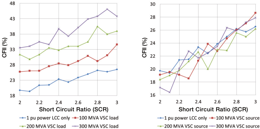
Figure 59 Comparison of CFI with Short Circuit Ratio Noting Influence of VSC as a Source or Load
