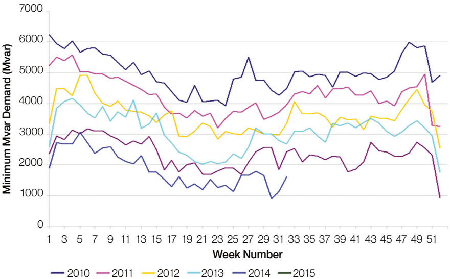
Figure 43 Actual Minimum MVar Demand
