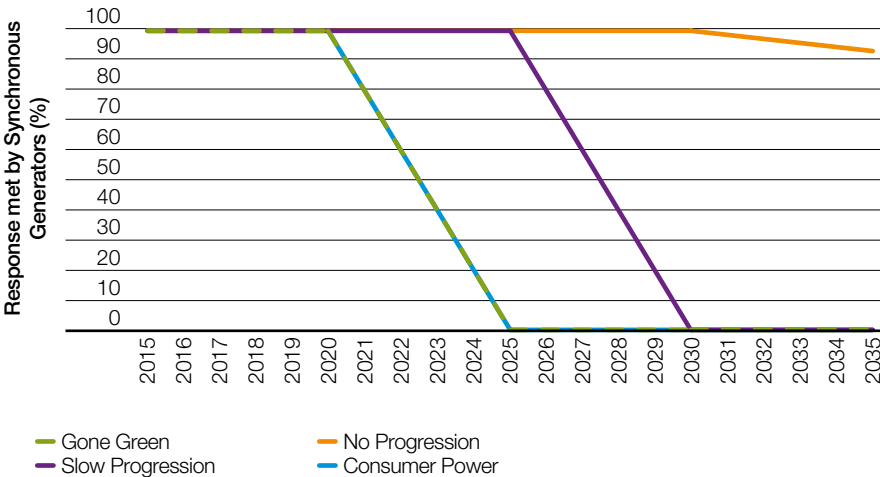
Figure 20 Percentage of Required Response that can be met by Operating Synchronous Generators
