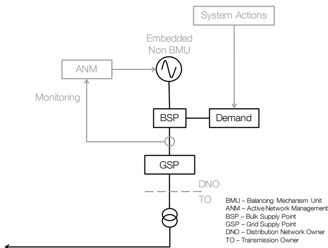
Figure 72 Type-A ANM Architecture
