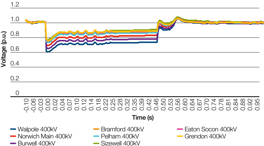
Figure 38 2025 Gone Green 3-phase to Earth Fault at Walpole 132kV Transient Voltage Dip Event
