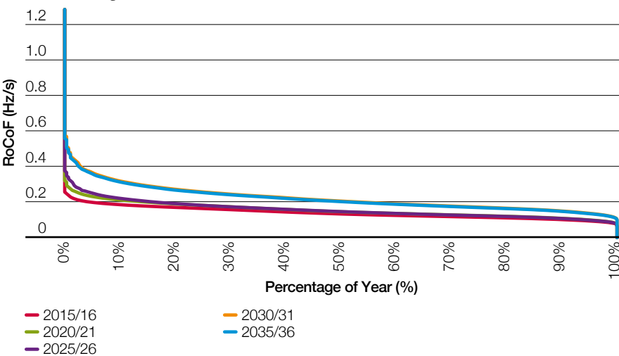
Figure 17 RoCoF – No Progression
