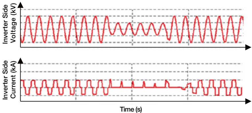
Figure 55 Illustrative LCC Type HVDC Commutation Failure
