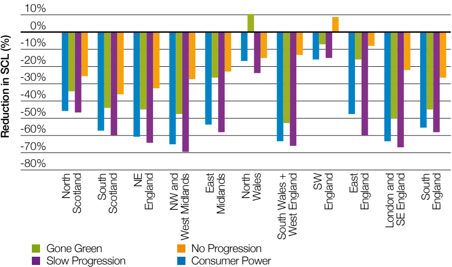
Figure 27 SOF 2015 Regions – SCL Decline 2035/26 vs 2015/16 Levels
