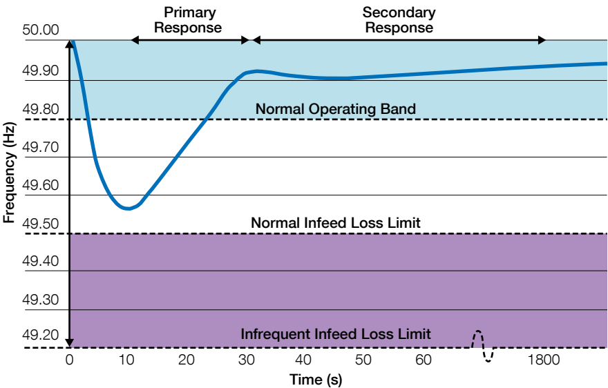
Figure 7 Illustrative Frequency Response Timescales
