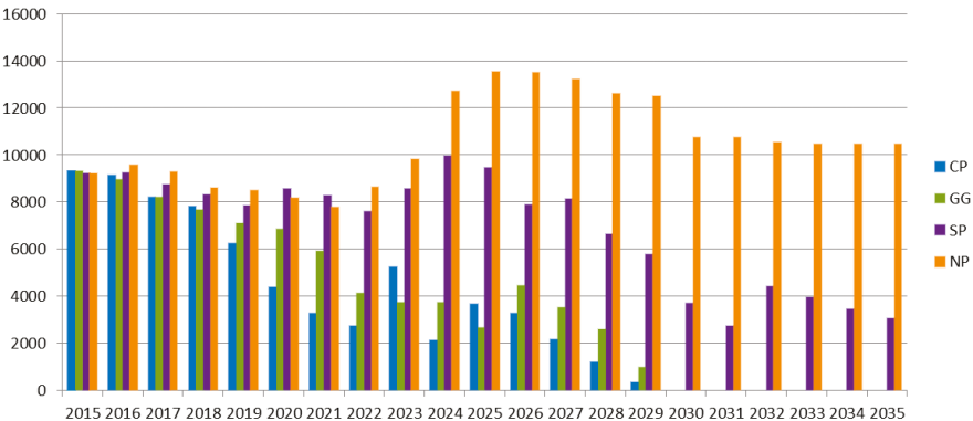
Figure 63 Transmission Connected Non-synchronous Generation Contribution at Minimum (Excluding HVDC)
