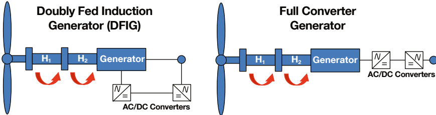
Figure 9 Wind Generation Technologies
