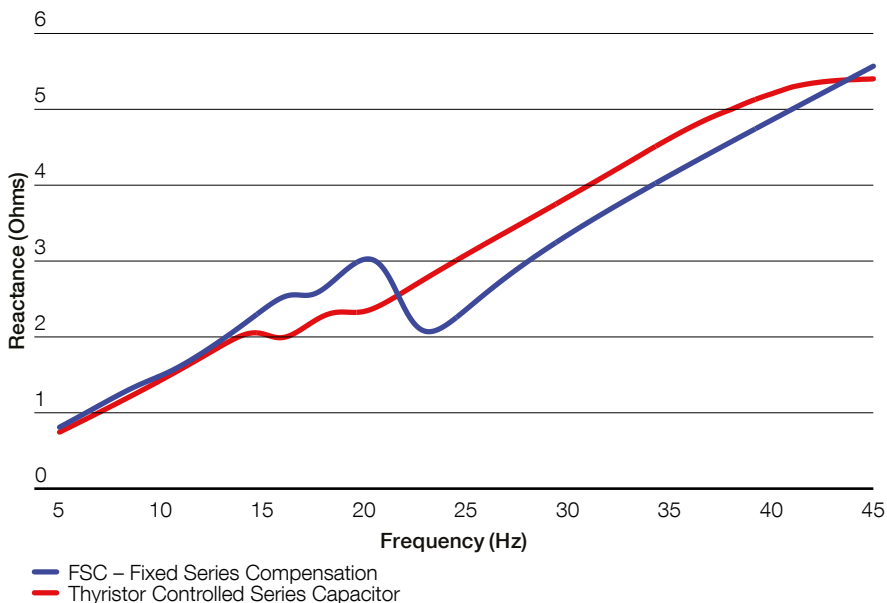
Figure 81 Frequency Scan of a Network with FSC (no SSR filter) and TCSC with SSR Control
