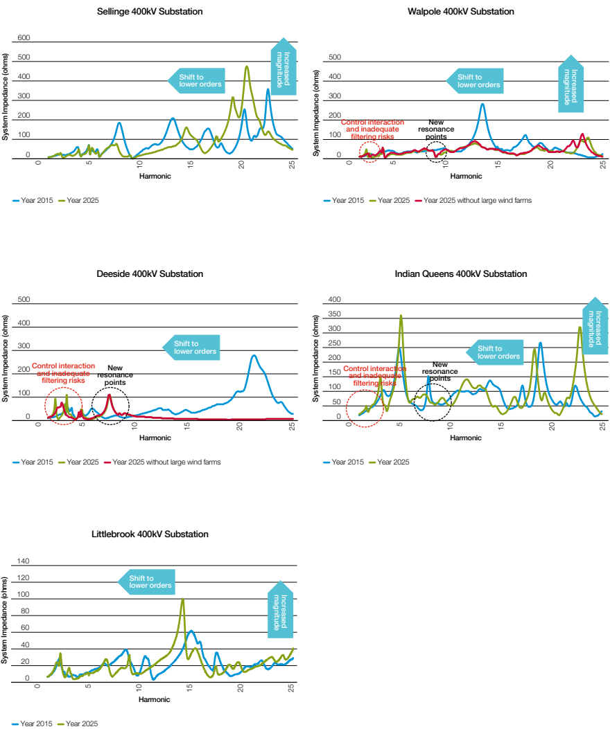
Figure 53 Frequency Scans up to 25th Harmonic Order in 2015 and 2025
