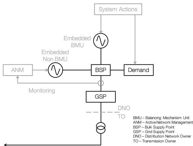
Figure 73 Type-B ANM Architecture
