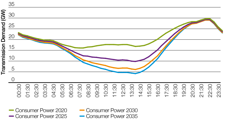
Figure 61A Summer Balancing Case Study With Proportions of Generation By Type (Chapter 7 FES 2015)
