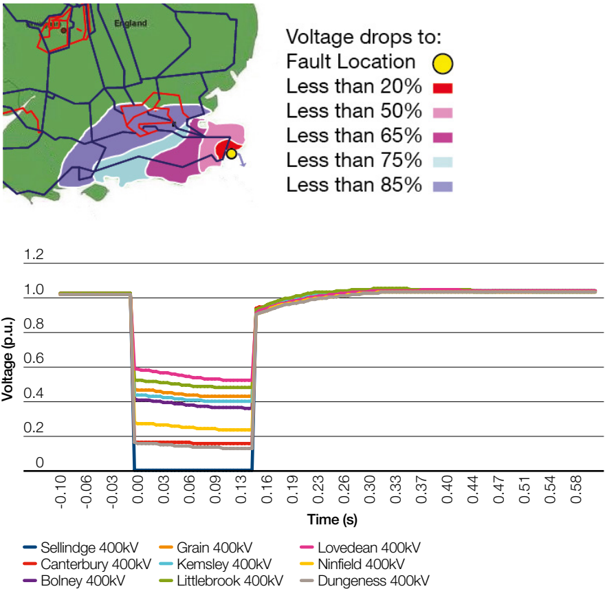
Figure 39 Current Network 3-phase to Earth Fault at Sellindge 400kV Voltage Dip for 140ms
