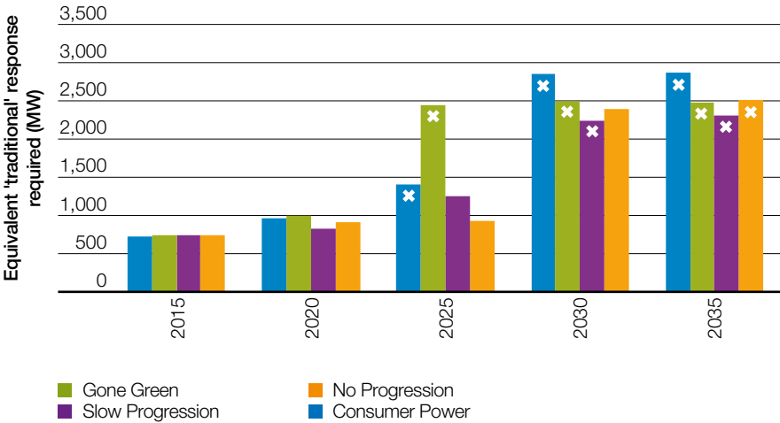
Figure 19 ‘Traditional’ Primary Frequency Response Required in the Absence of Alternatives
