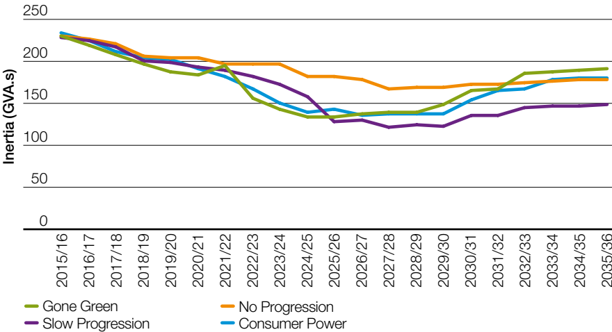
Figure 12 Minimum System Inertia Including Contribution from Embedded Generation
