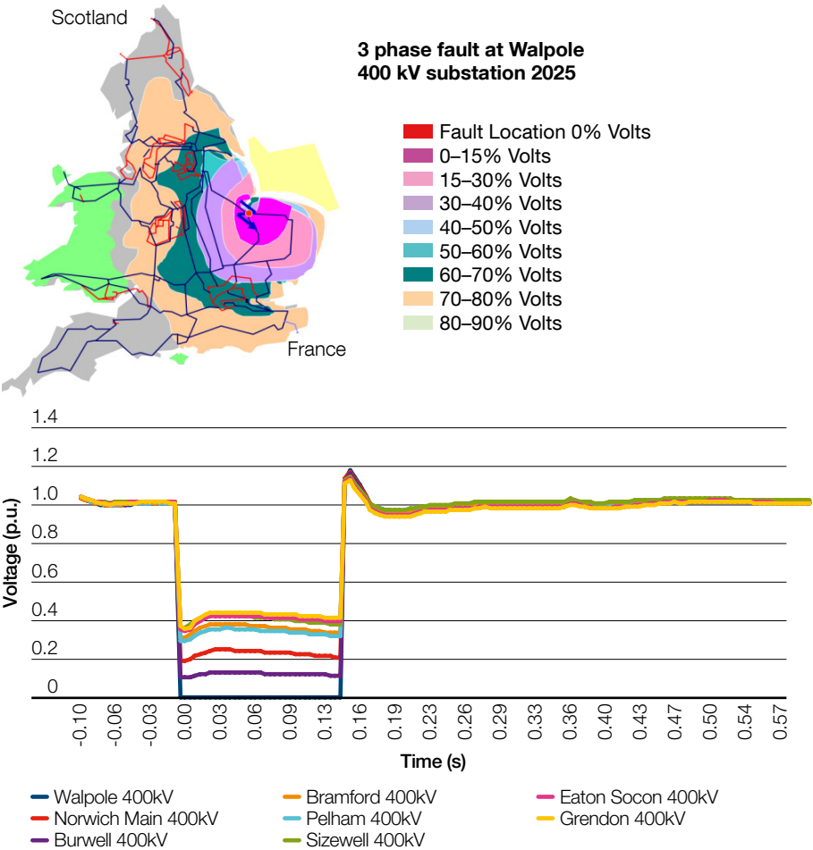
Figure 32 2025 Gone Green Effect of 3-phase Earth Fault at Walpole 400kV
