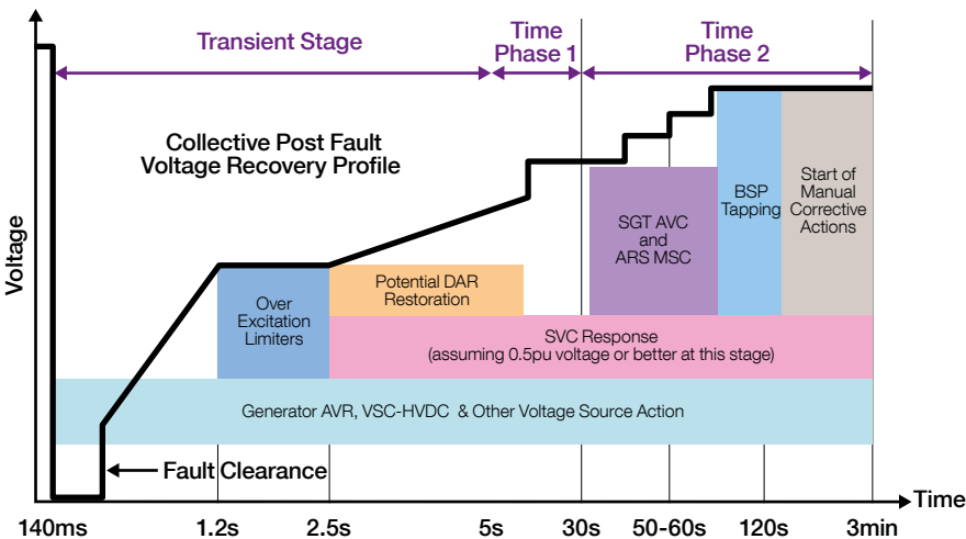
Figure 30 The Collective Post Fault Voltage Recovery and Influencing Factors
