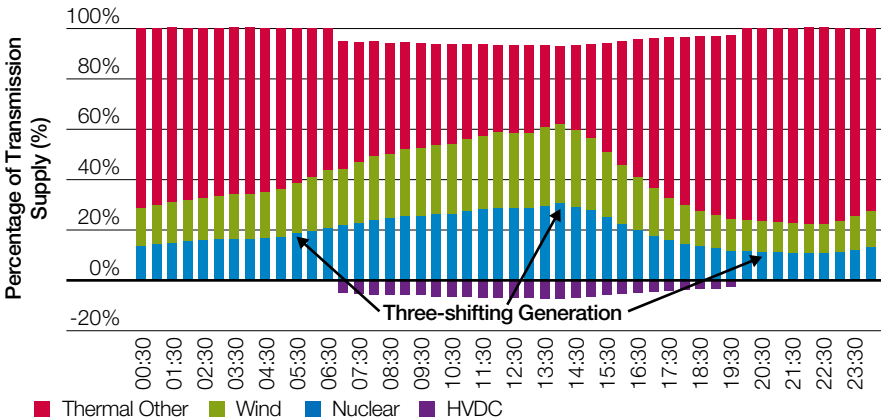
Figure 61C Summer Balancing Case Study With Proportions of Generation By Type (Chapter 7 FES 2015)
