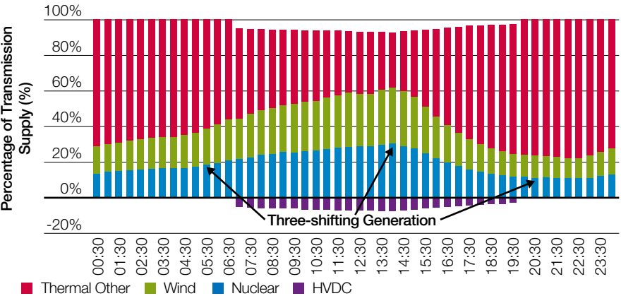
Figure 28B 2025 Thermal Generation Shifting Against FES 2015 Balancing Case Study
