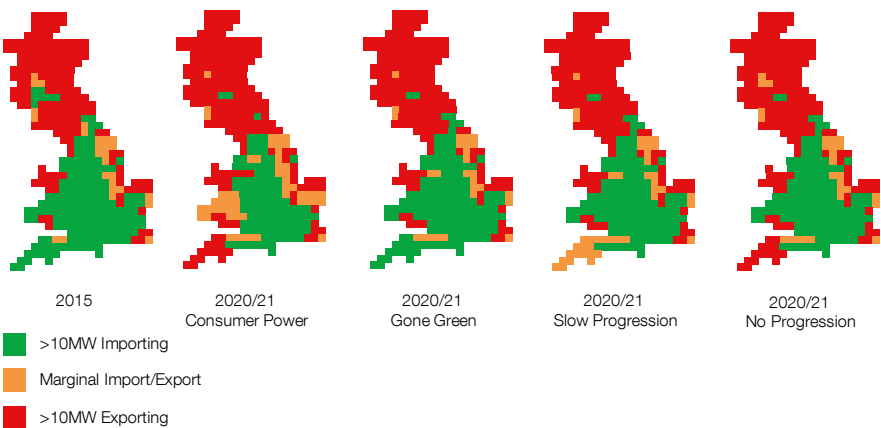
Figure 71 GSPs Expected to Be Exporting Active Power at Some Point During the Year
