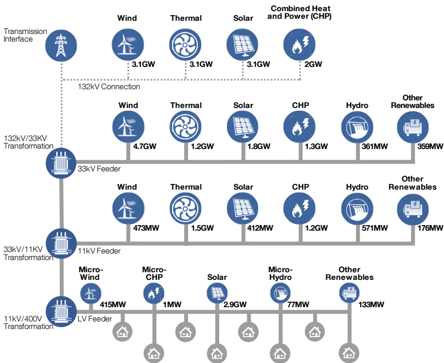
Figure 69 Embedded Generation Total Capacities and Location in GB
