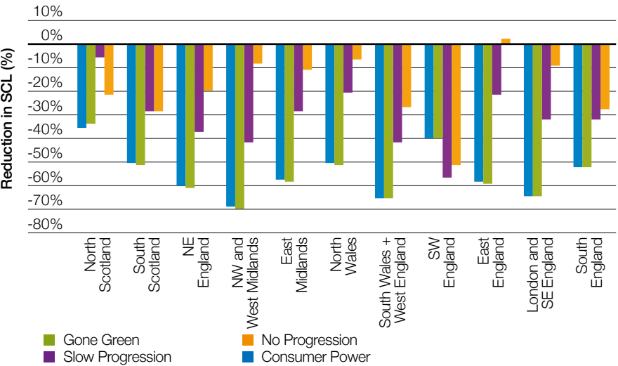
Figure 26 SOF 2015 Regions – SCL Decline 2025/26 vs 2015/16 Levels
