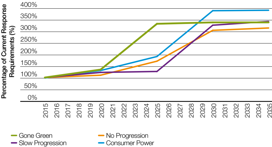
Figure 18 Summer Minimum Primary Response Requirements as a Percentage of 2015 Requirements
