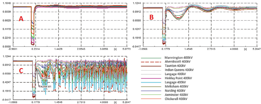
Figure 67 Changing System Response Dependent on Level of Embedded Generation
