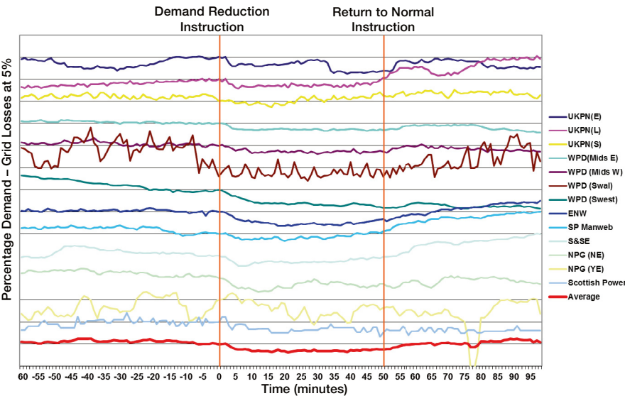
Figure 60 Change in Load by DNO Area As Observed in Operation Juniper Demand Control by Voltage Reduction Trial
