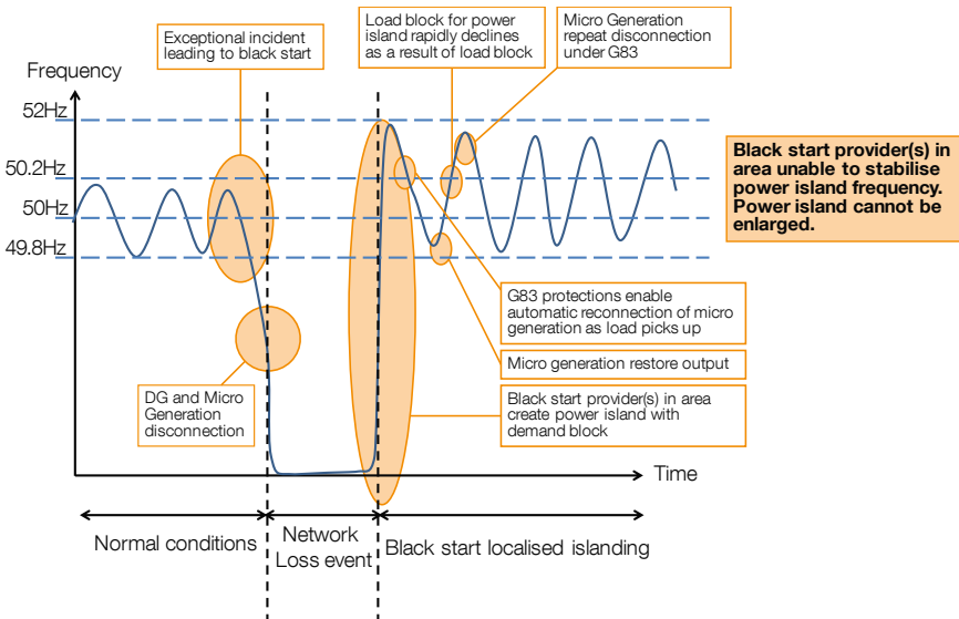
Figure 64 Stability Concern Surrounding Stability of Block Loads during Black Start Events
