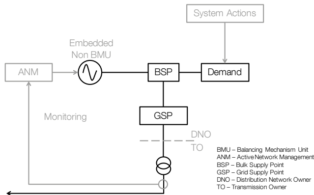
Figure 74 Type-C ANM Architecture
