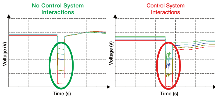
Figure 83 Control System Interaction
