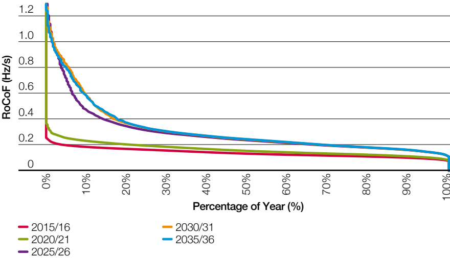
Figure 16 RoCoF – Slow Progression
