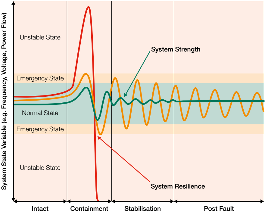
Figure 10 System Strength and Resilience Relating to a Disturbance
