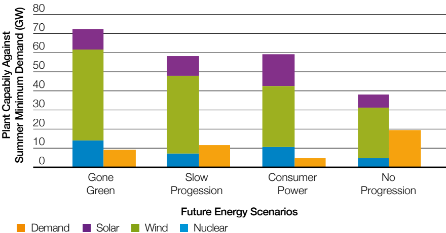
Figure 84 Summer Minimum 2035/36 Plant Capabilities and Demand
