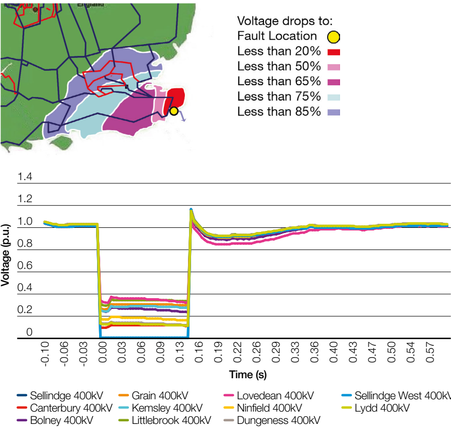
Figure 40 2025 Gone Green 3-phase to Earth Fault at Sellindge 400kV Transient Voltage Dip for 140ms
