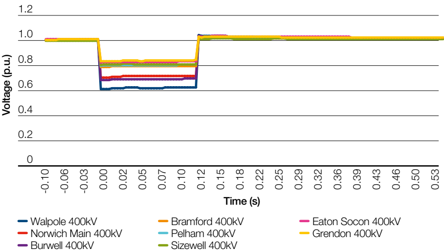
Figure 35 Current Network 1-phase to Earth Fault at Walpole 400kV Transient Voltage Dip Event
