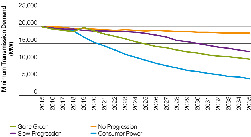
Figure 23 Minimum Transmission System Demand at GSP Interface
