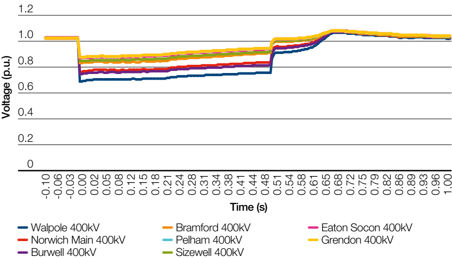
Figure 37 Current Network 3-phase to Earth Fault at Walpole 132kV Transient Voltage Dip Event
