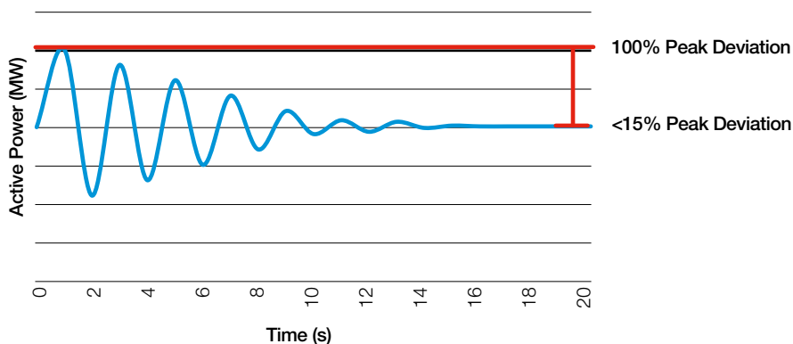
Figure 65 NETS SQSS Power Oscillation Damping Requirement
