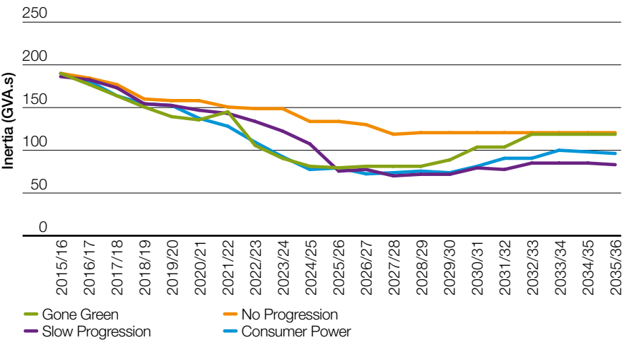
Figure 13 Minimum System Inertia Excluding Contribution from Embedded Generation
