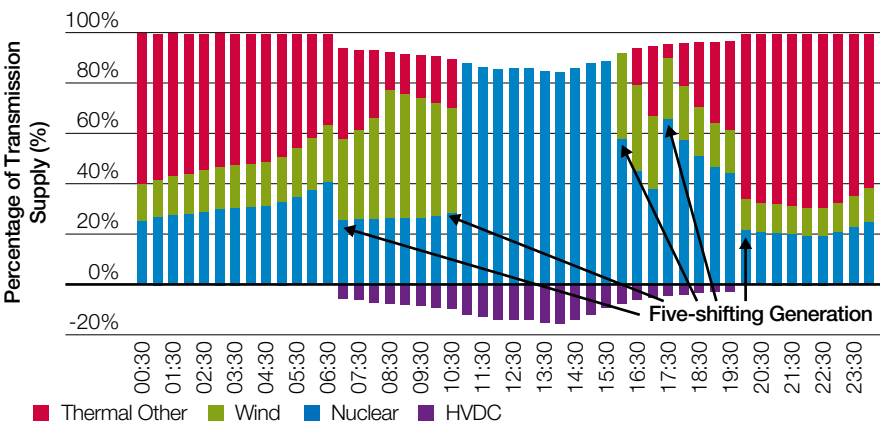
Figure 61D Summer Balancing Case Study With Proportions of Generation By Type (Chapter 7 FES 2015)
