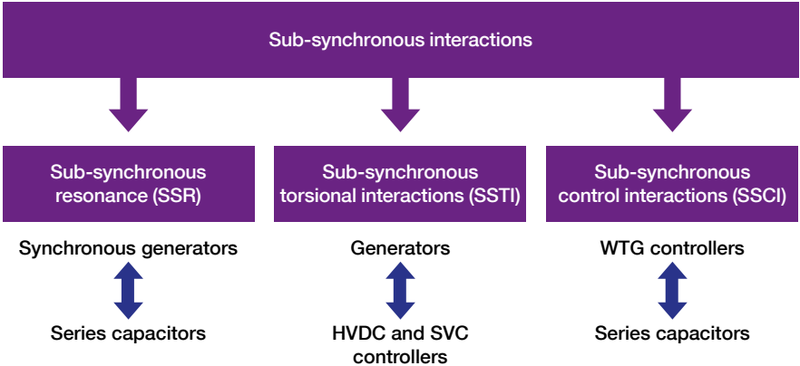
Figure 80 Sub-synchronous Interaction Classification
