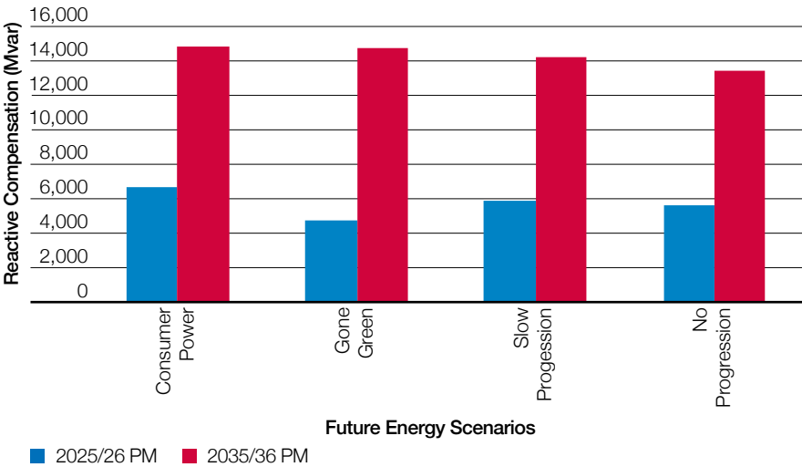
Figure 50 Reactive Compensation Required to Contain Transmission System Voltage
