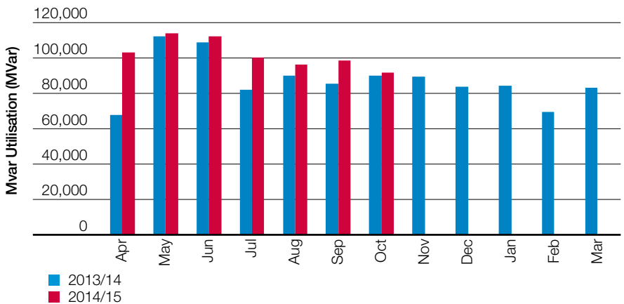
Figure 45 Mvar Utilisation Over Recent Years
