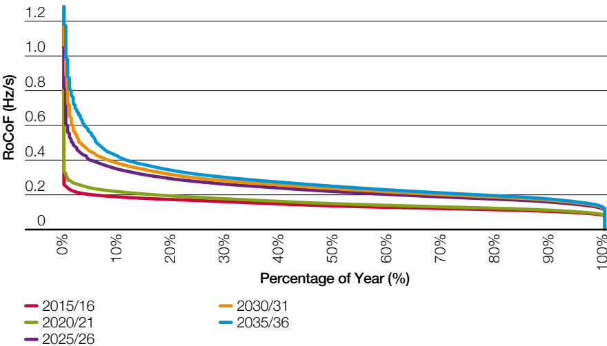
Figure 14 RoCoF – Consumer Power
