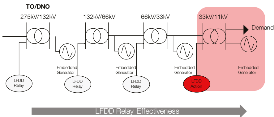
Figure 68 LFDD Preferred Operation Point
